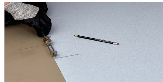
Figure 14 Scribing the wall profile
