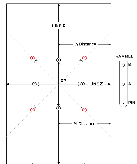
Figure 7 Marking out diagonal tiling
